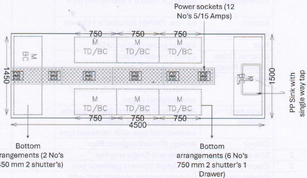
Rough sketch/ drawing of modular island bench
