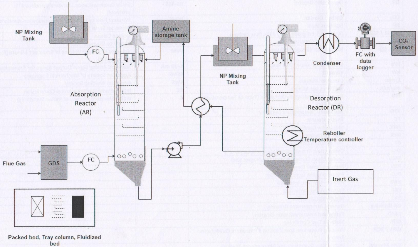
Process Flow Diagram for proposed capture system
